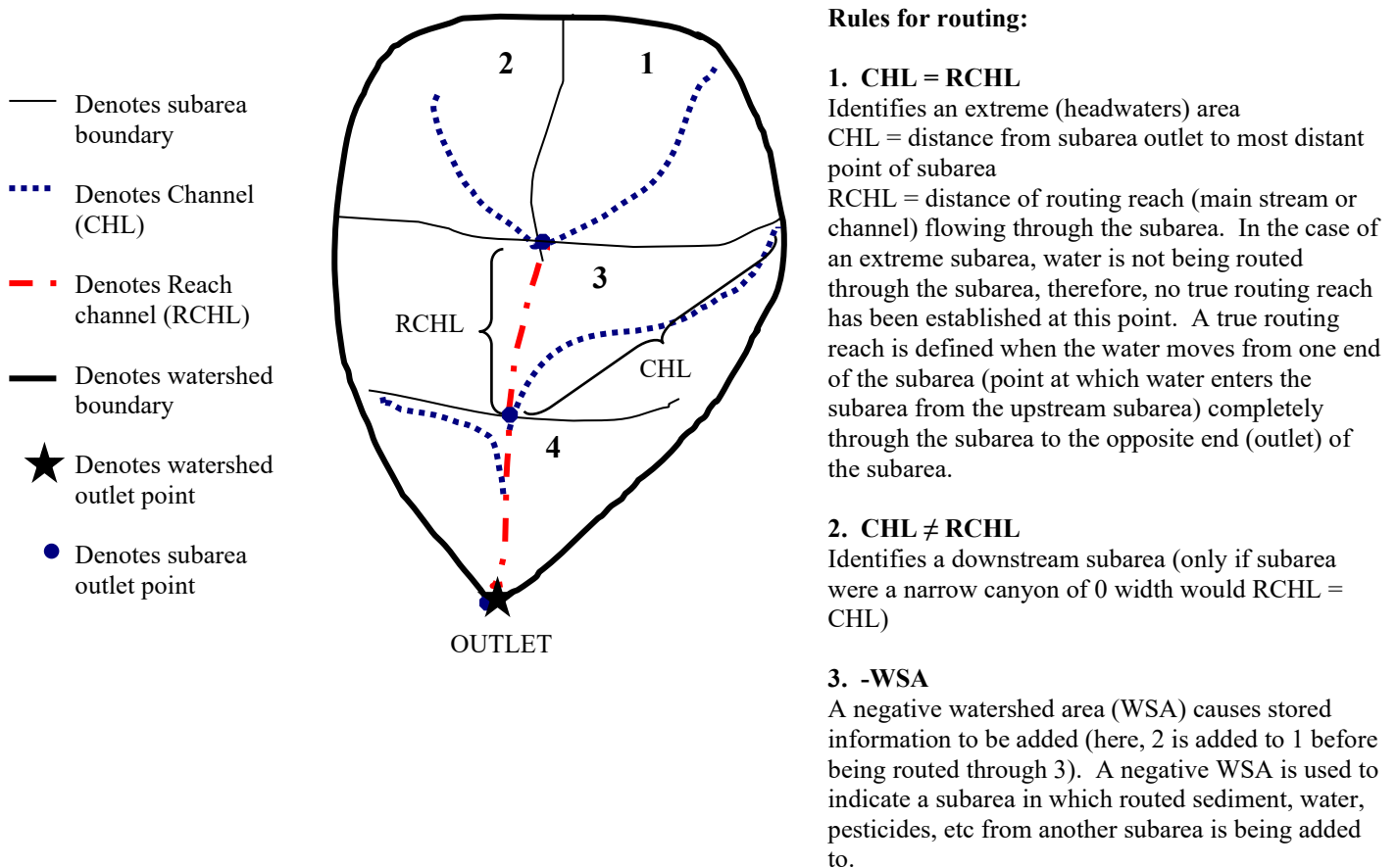
Figure 2.5: Illustration of a watershed and rules for using the routing mechanism in APEX
