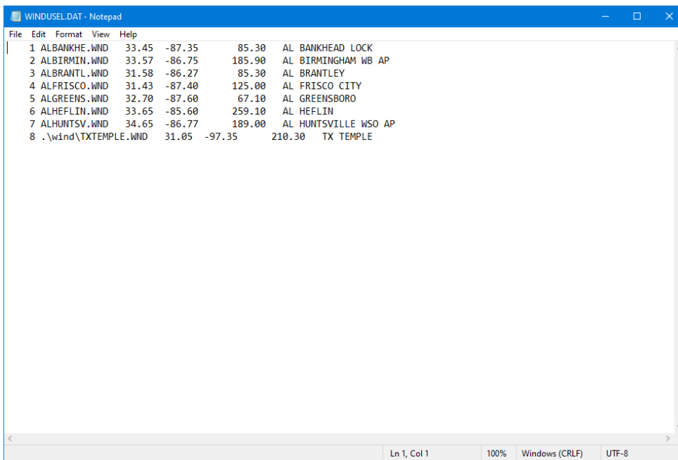
Figure 14. Example of EPIC wind data list file. In this example, the wind data files from 1 to 7 are in the same directory of the EPIC executable while the wind data file "TXTEMPLE.WND" is in the folder "wind" which is located in the same folder where the EPIC executable is.
